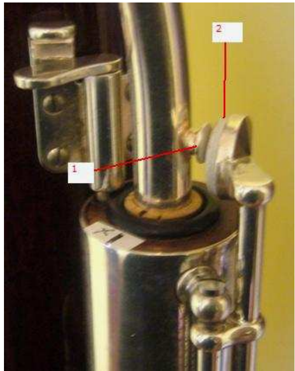
Octave bush (1) covered by pad (2)
